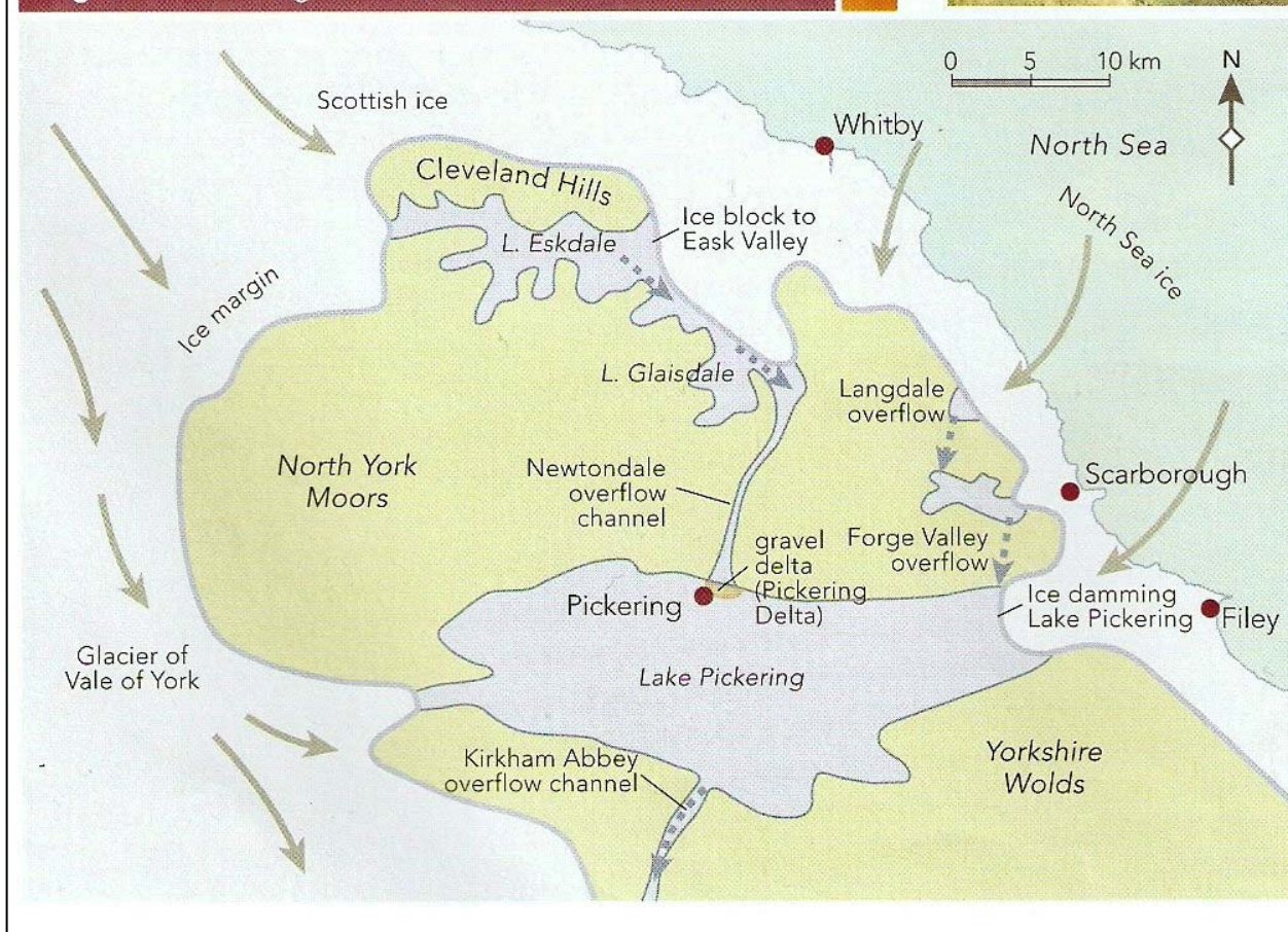
Figure 3.17 Drainage modification in the North York Moors
